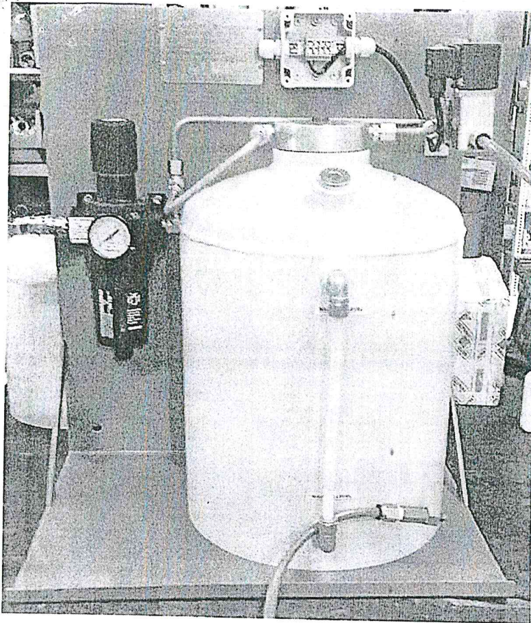
SPRAY SYSTEM WITH 23 LITRE RESERVIOR AND SPRAY CONTROL VALVE, SOLENIOD VALVE AND SINGLE NOZZLE
