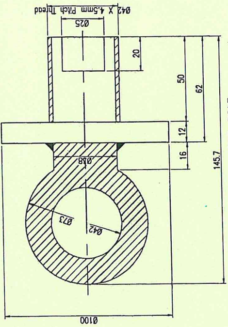
EYE-BOLT
