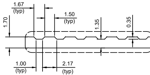
DETAIL "A" 1:3
