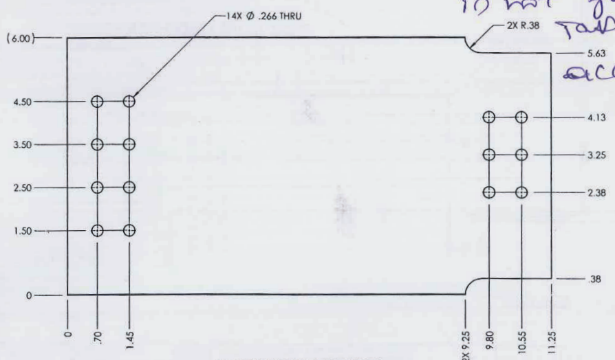
75352113-101-101 STIFFENER FRONT VIEW
