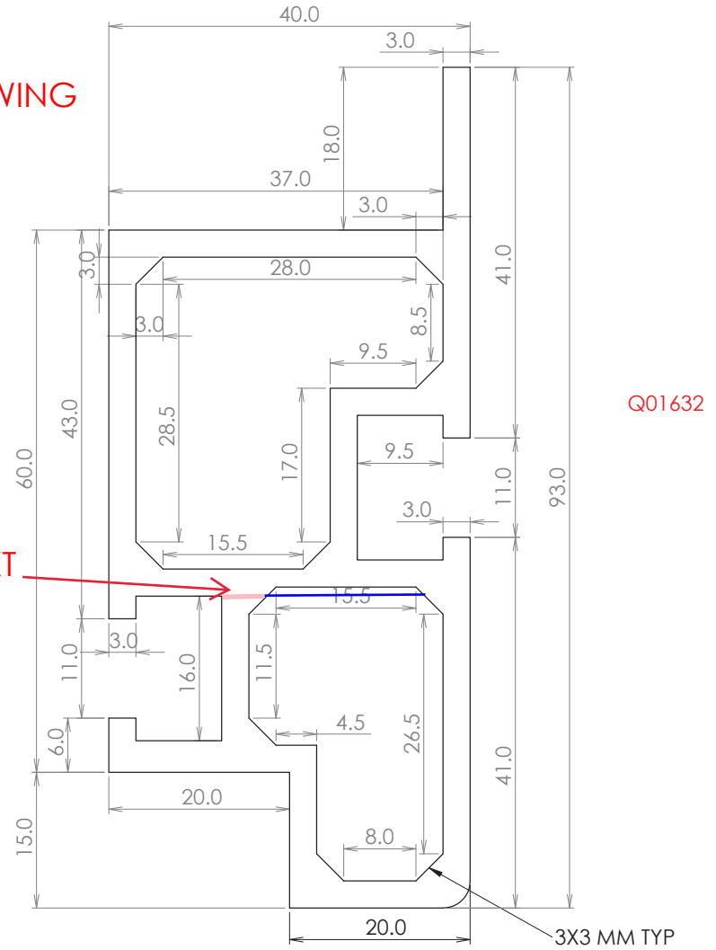
PROFILE-2
