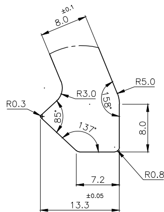
SECTION: X-X'
