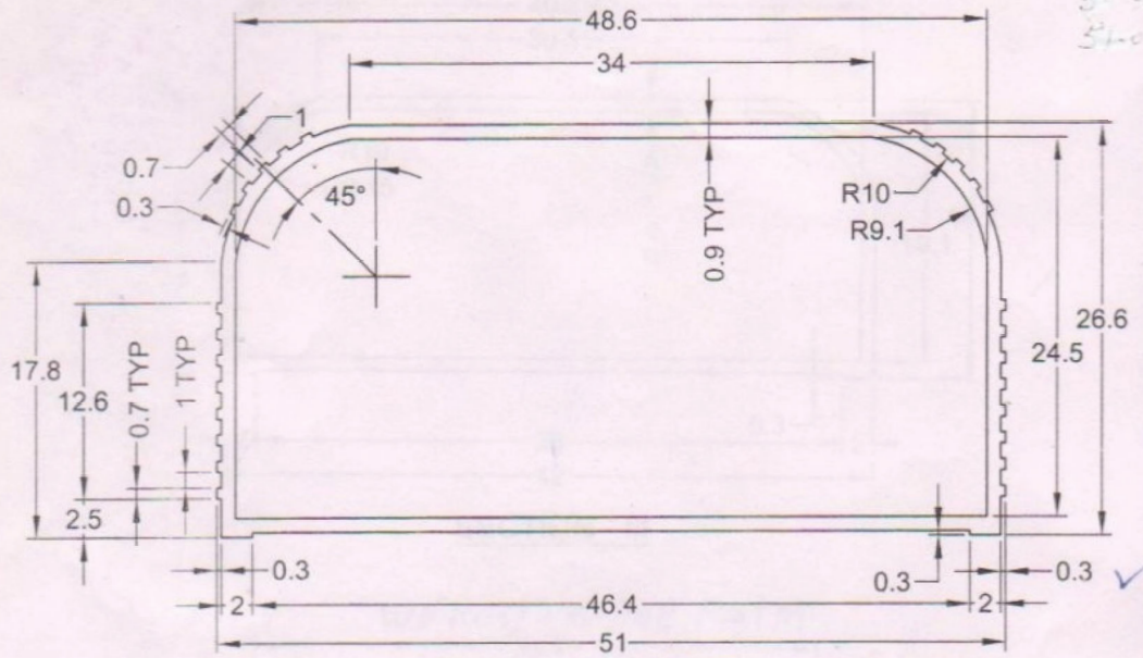
SECTION - I
