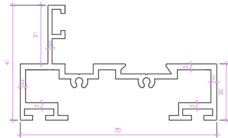
WINDOW OUTER FRAME SECTION DETAILS
