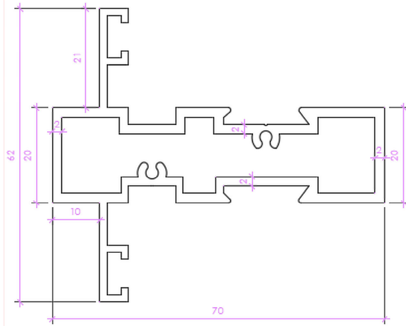
WINDOW MIDDLE FRAME SECTION DETAILS
