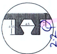
Section-B
