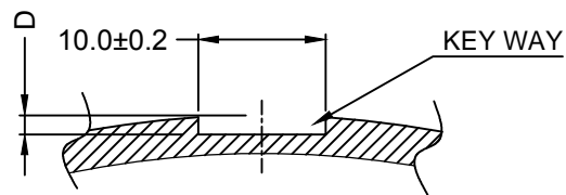
SECTION -C (2 Key Way)
