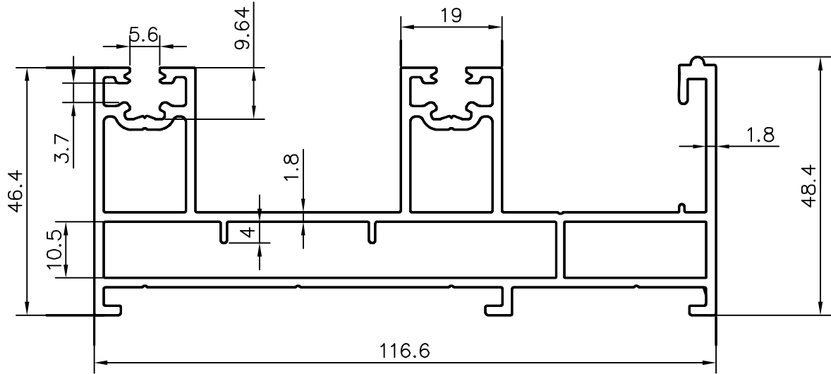
84120 2TARCK SLIDING FRAME
