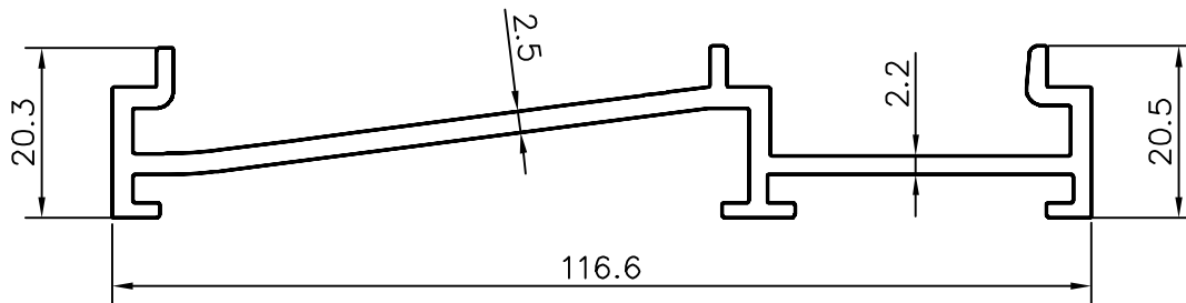
84702 2TRACK FRAME BOTTOM CLIP
