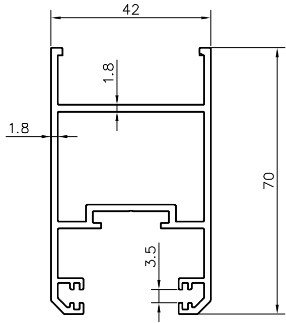
84216 HANDLE SECTION SASH
