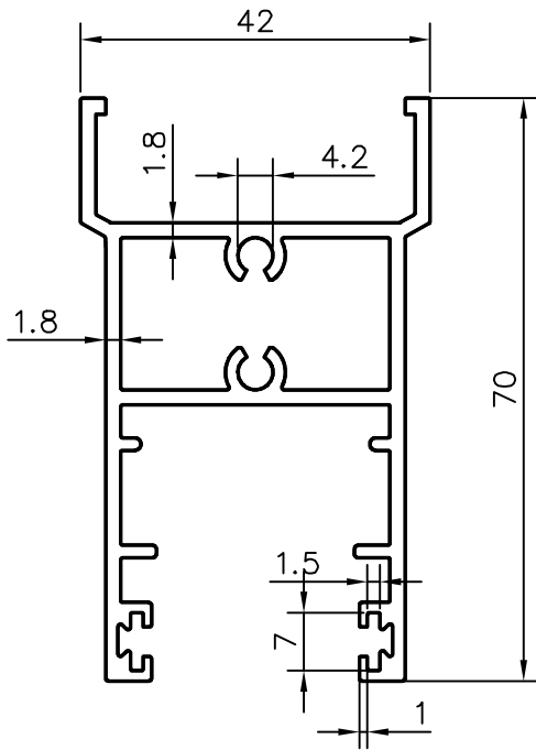
84217 HORIZONTAL SASH
