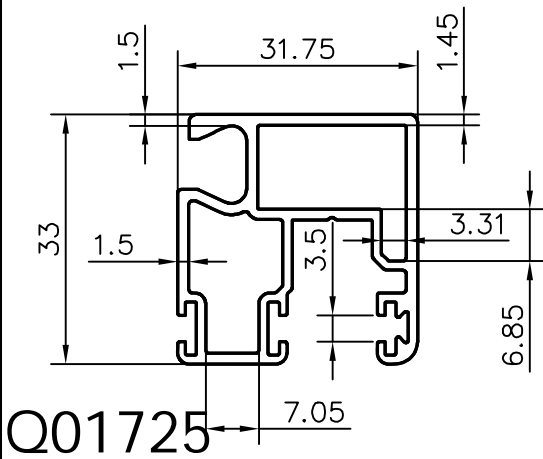
84218 MESH SASH PROFILE
