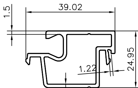
84512 MESH ADAPTOR
