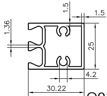
84304 MESH MULLION PROFILE
