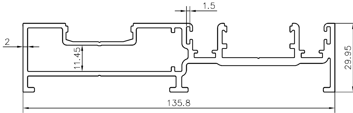
2 Track Vertical Frame Profile
