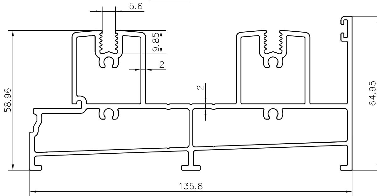
2 Track Horizontal Frame Profile
