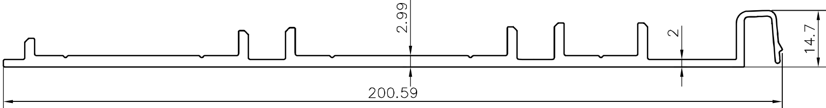
84811 3 Track Installer Base Clip
