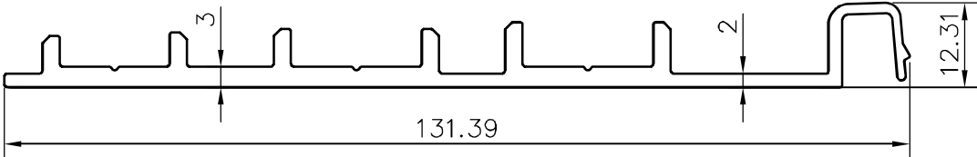
84812 2 Track Installer Base Clip
