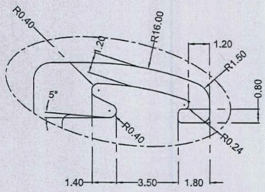
DETAILS A SCALE 1 : 2.5
