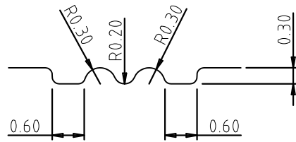
Scale = 10:1 BHORUKA ID MARK - TYPE 2
