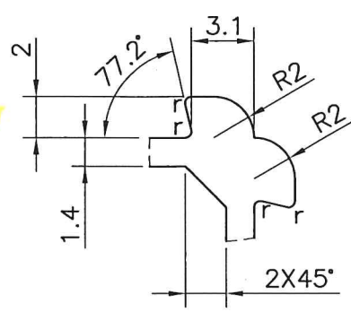
DETAIL B SCALE 3:1
