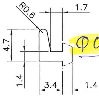
DETAIL A SCALE 3:1
