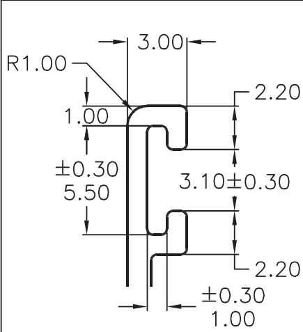
DETAILS:- A SCALE:- 4:1
