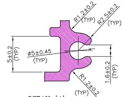
DETAIL-'A' SCALE 4:1
