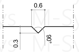
Detail @ 'V' Groove
