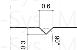
Detail @ 'V' Groove
