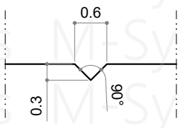
Detail @ 'V' Groove
