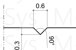
Detail @ 'V' Groove
