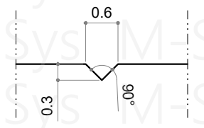
Detail @ 'V' Groove
