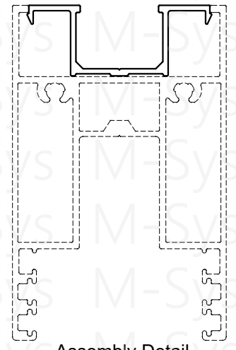
Assembly Detail
