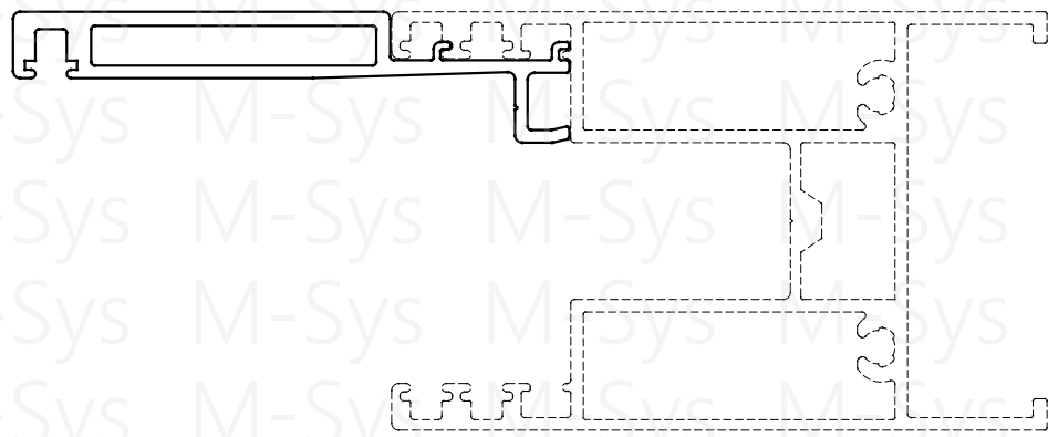
Assembly Detail
