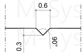
Detail @ 'V' Groove
