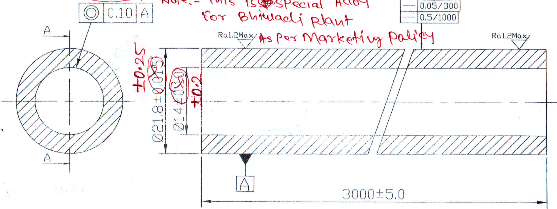
Section- A-A
