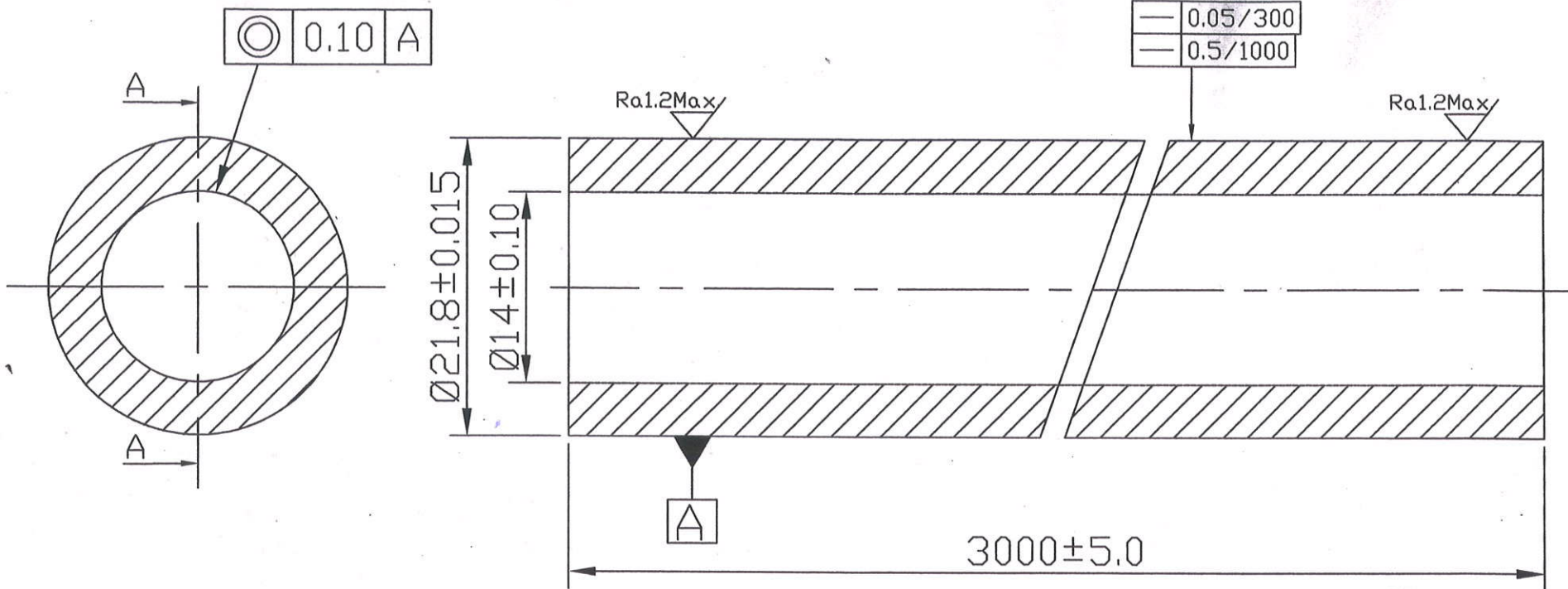
Section- A-A
