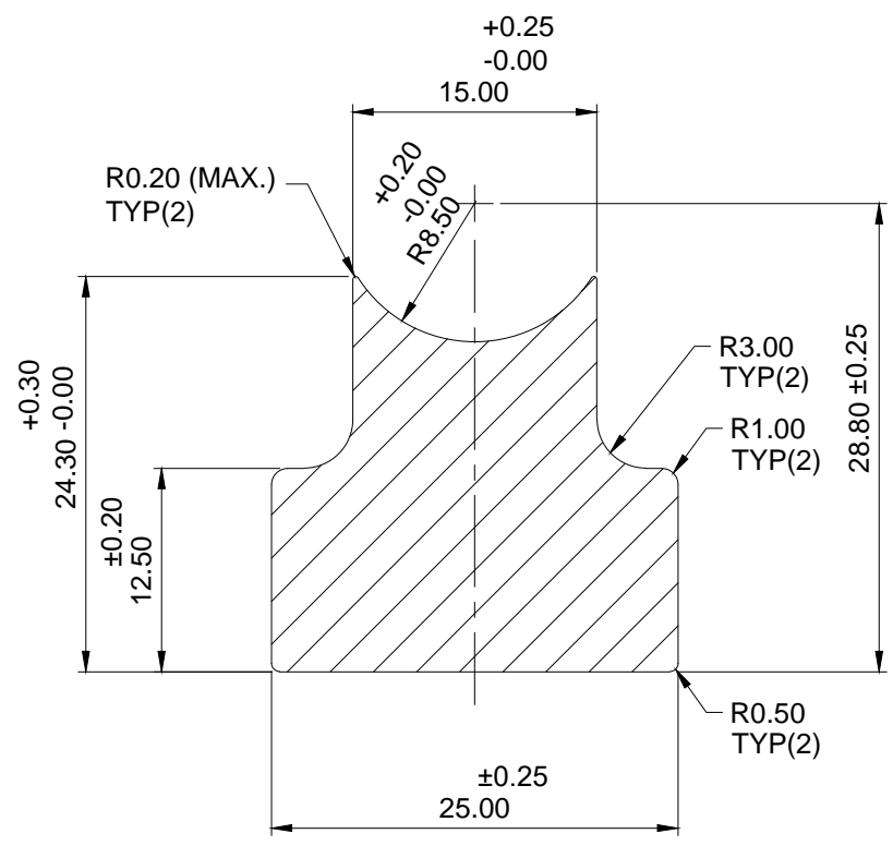
DETAILED SECTION DRAWING (SCALE - 2 : 1)
