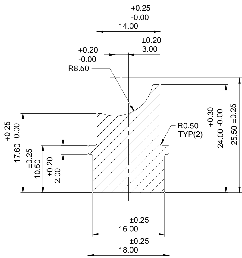
DETAILED SECTION DRAWING (SCALE - 2 : 1)
