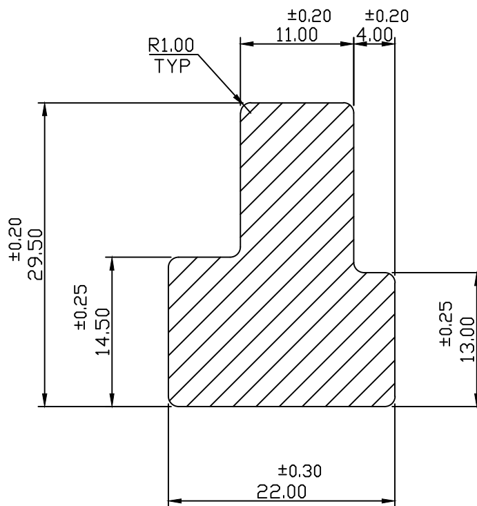
DETAILED SECTION DRAWING (SCALE - 2 : 1)
