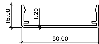
MULLION COVER CAP
