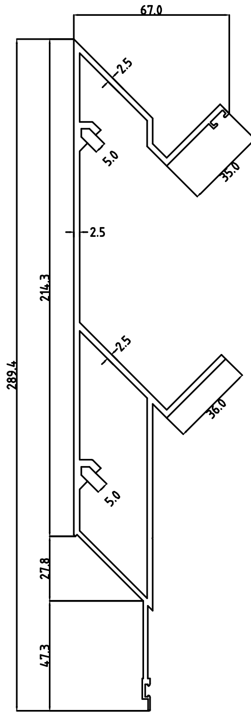
CORNER MALE MULLION
