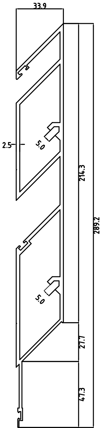
CORNER FEMALE MULLION
