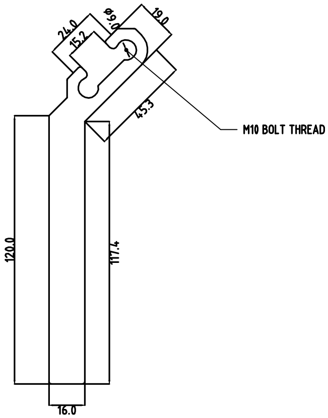
ALUM. HOOK BRACKET ELEMENT - 4
