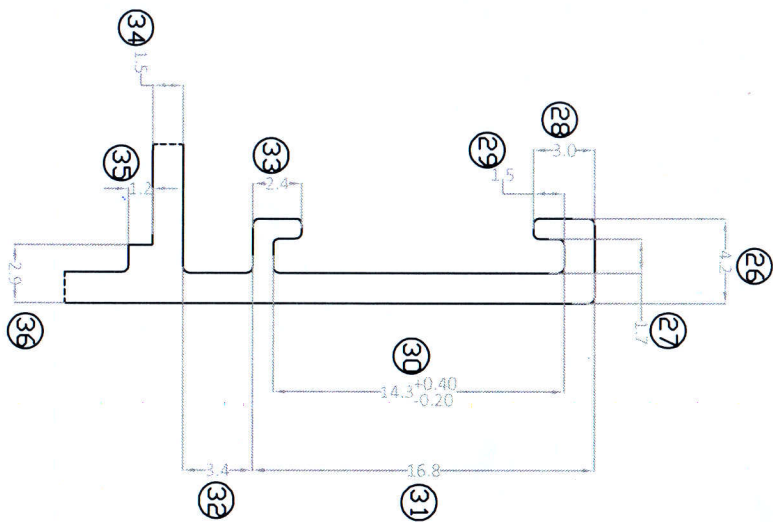
SECTION B-SCALE-5:1
