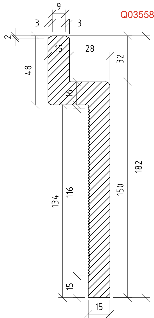
FACE MOUNTED BRACKET
