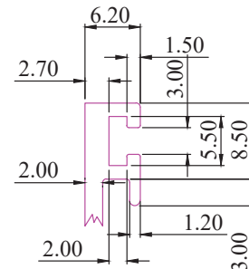
DETAILS 'C' SCALE-2:1
