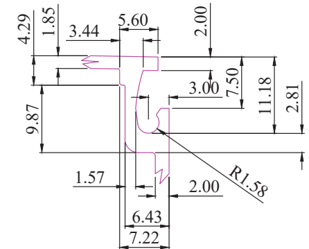
DETAILS 'A' SCALE-2:1
