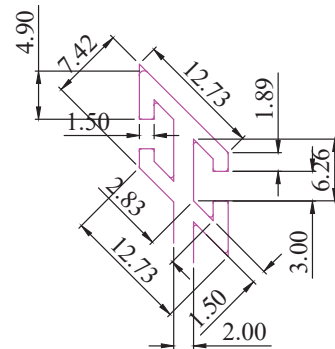
DETAILS 'C' SCALE-2:1
