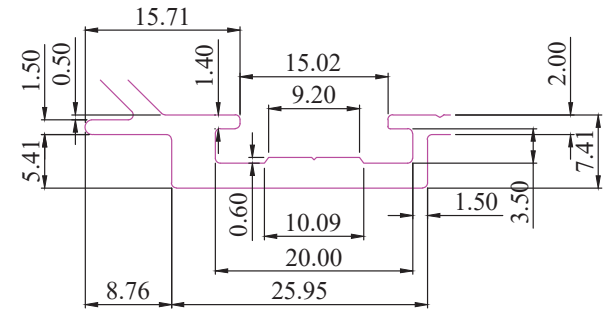
DETAILS 'B' SCALE-2:1
