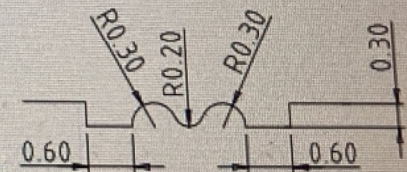
DETAIL-A BHORUKA ID MARK - TYPE 2 SCALE-10:1
