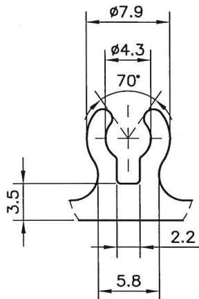
DETAIL A SCALE 2:1
