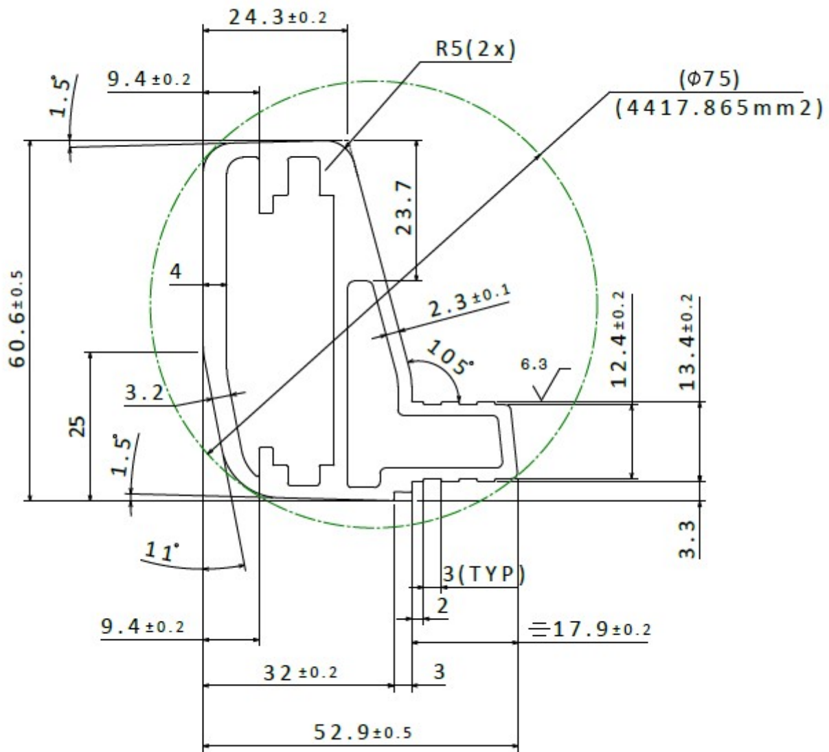
Front view[6] Scale: 2:1
