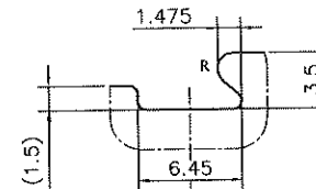
DETAIL B SCALE 3:1
