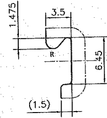
DETAIL A SCALE 3:1
