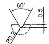
DETAIL V SCALE 4:1
