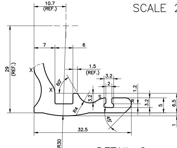
DETAIL C SCALE 2:1
