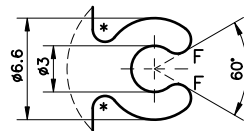
DETAIL B SCALE 3:1
