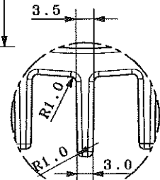
DETAIL G SCALE 1:1
