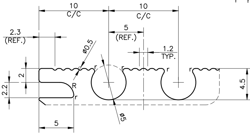
DETAIL A SCALE 3:1
