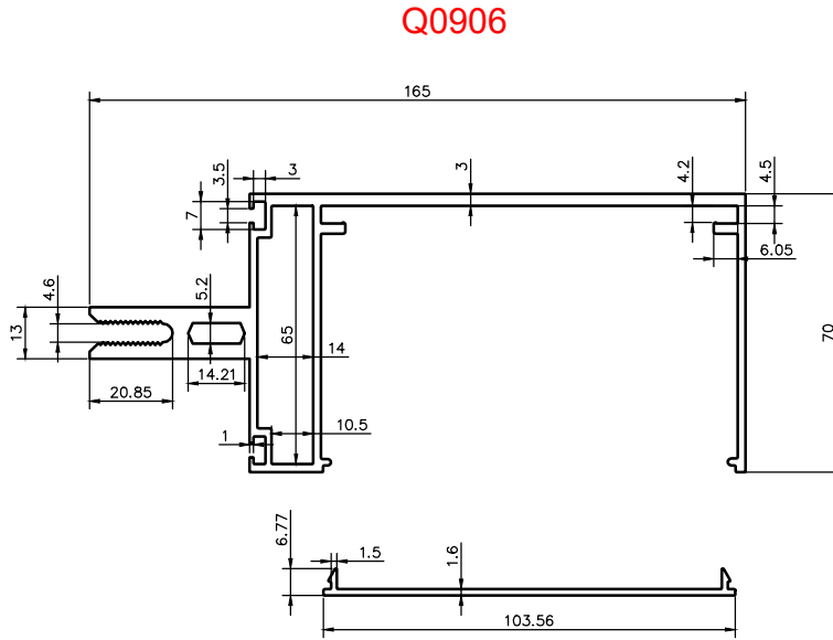
TRANSOM PROFILE
