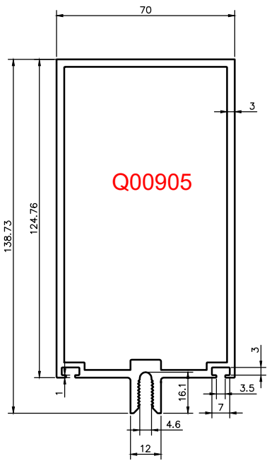
MULLION PROFILE
