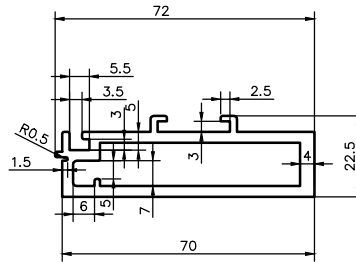
SHUTTER PROFILE
