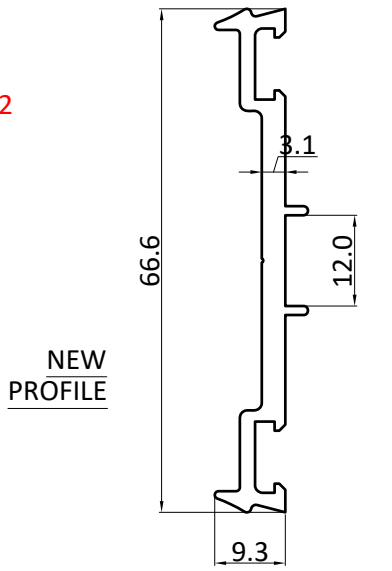
PRESSURE PLATE PROFILE
