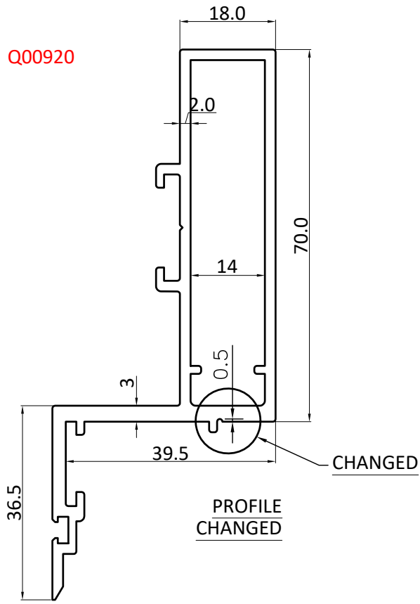
SHUTTER PROFILE
