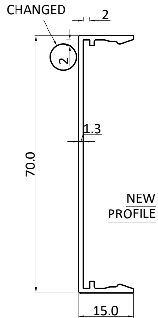
COVER PLATE PROFILE
