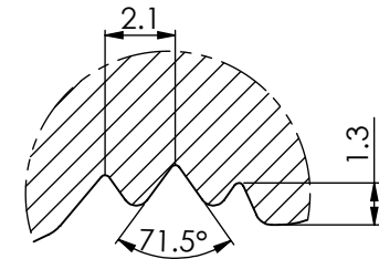
DETAIL X
